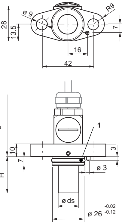
Cable end: flying lead
