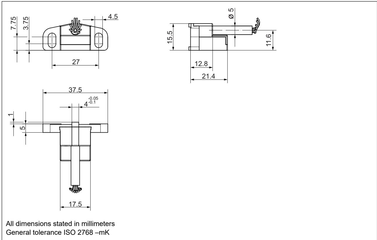
Dimensional drawing GEL 2444 with cable outlet MiniCODER (L) — tangential left
