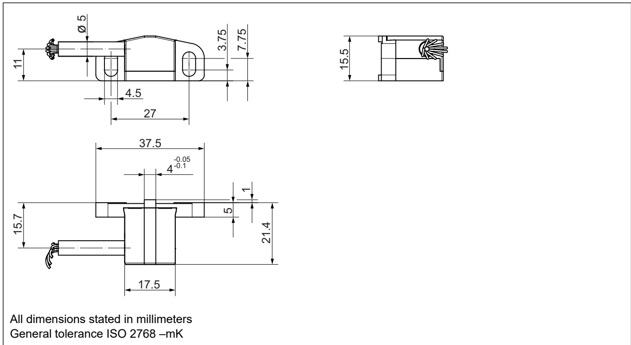
Dimensional drawing GEL 2444 with cable outlet MiniCODER (L) — tangential left
